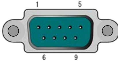
Output connector of PL20C
