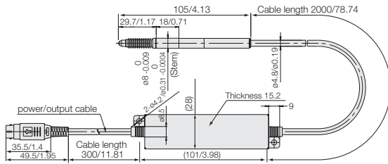
DK812AR/DK812AR5/DK812BR/DK812BR5
