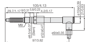
DK812AFLR/DK812AFLR5 DK812ABL/DK812BFLR5
