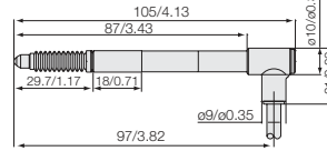
DK812ALR/DK812ALR5/DK812BLR/ DK812BLR5
